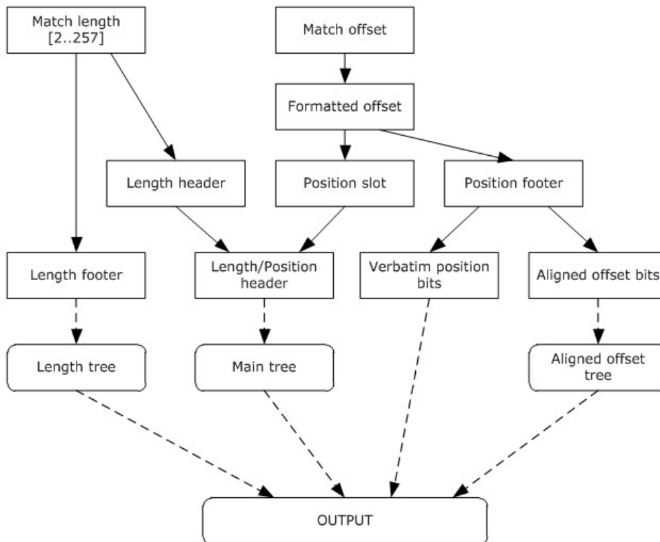
Figure 1: Match encoding subcomponents
